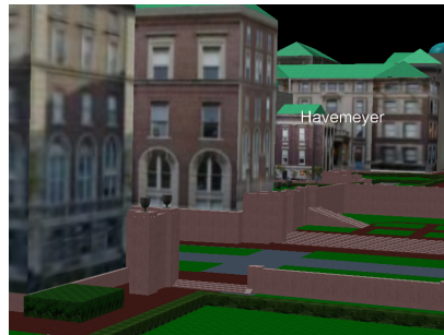
Figure 7. Area feature labeling comparison. (a) Naïve label placement at projected centroid of each building causes overlaps, and mislabeling because of buildings hidden partially or entirely. (b) Suppression of labels for buildings whose projected centroid is not visible. (c) Label placement using approach of Section 4.3.
